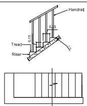
STAIRCASE DETAIL
