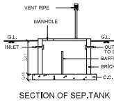
SECTION OF SEP.TANK
