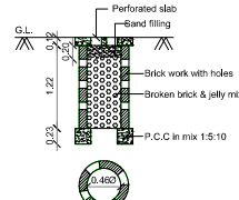
PERCOLATION PIT FOR 30 Sq. m. (Scale:- 1:50)
