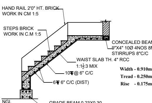
STAIRCASE DETAILS (SCALE 1:50)
