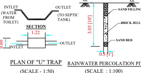
RAINWATER PERCOLATION PIT (SCALE : 1:100)
