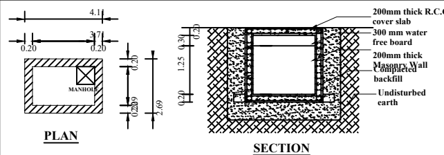
UNDERGROUND SUMP DETAIL (SCALE:1:100)
