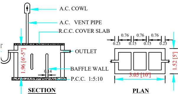
SEPTIC TANK DETAILS (SCALE:1:100)
