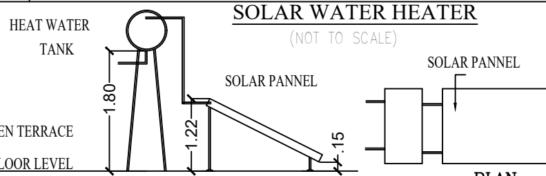
SOLAR WATER HEATER
