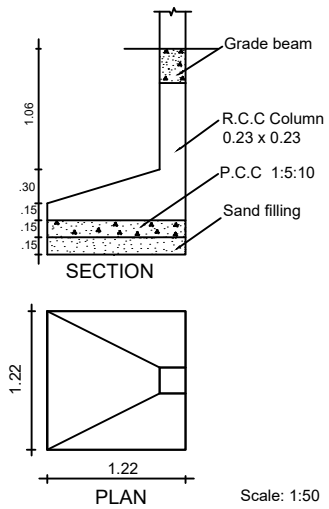
FOUNDATION DTAILS
