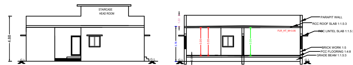
SECTION ON 'AB'
