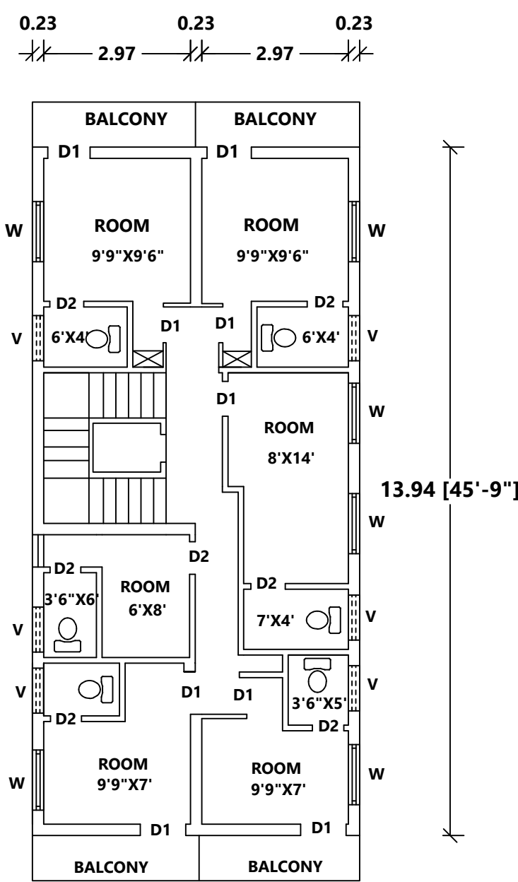
FLOOR 01
