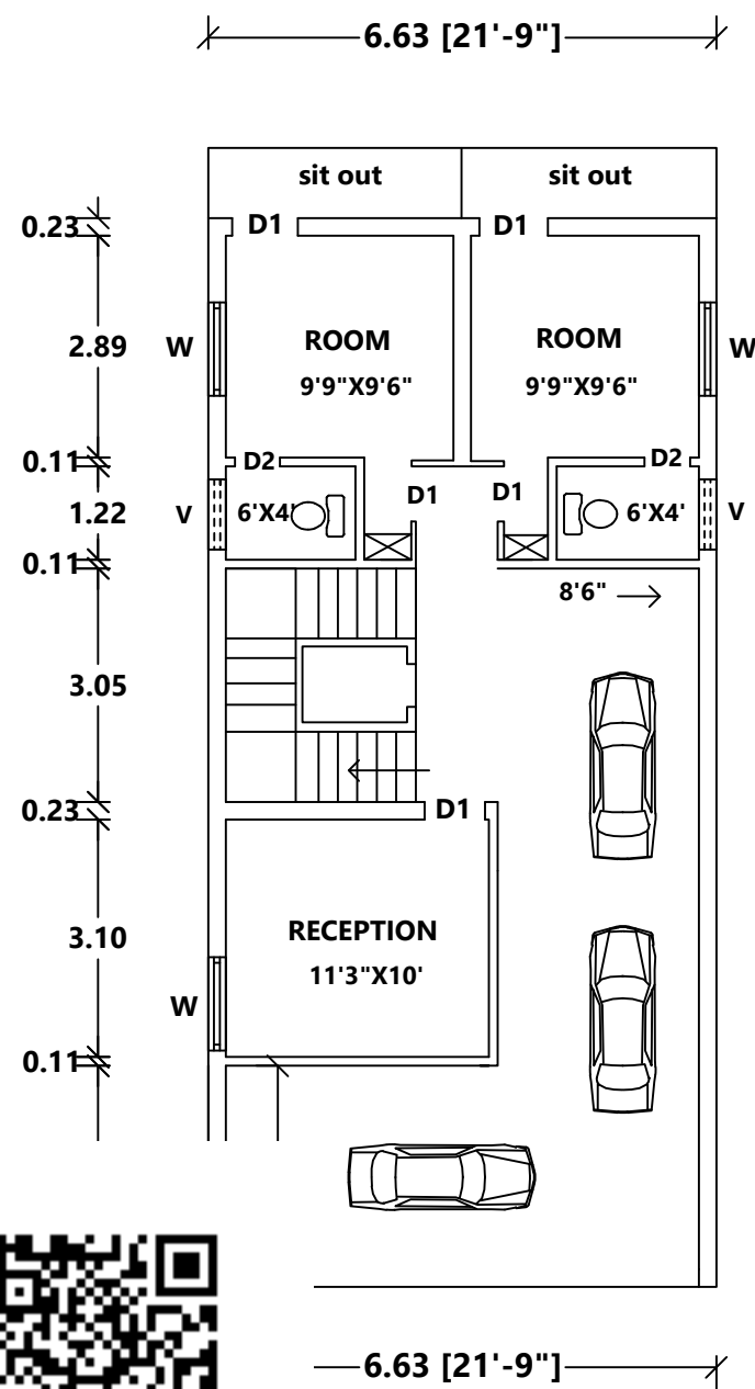
FLOOR GROUND
