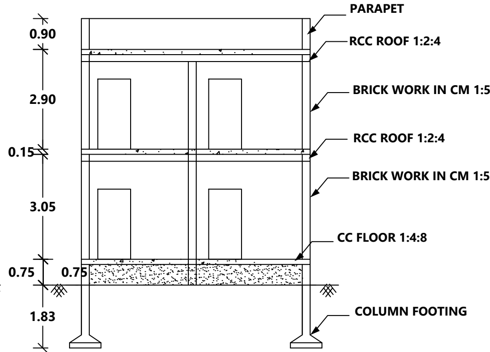
SECTION AB
