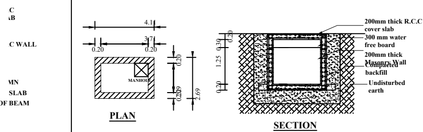
UNDERGROUND SUMP DETAIL (SCALE-1:100)
