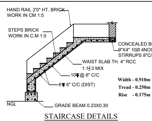
STAIRCASE DETAILS (SCALE 1:50)
