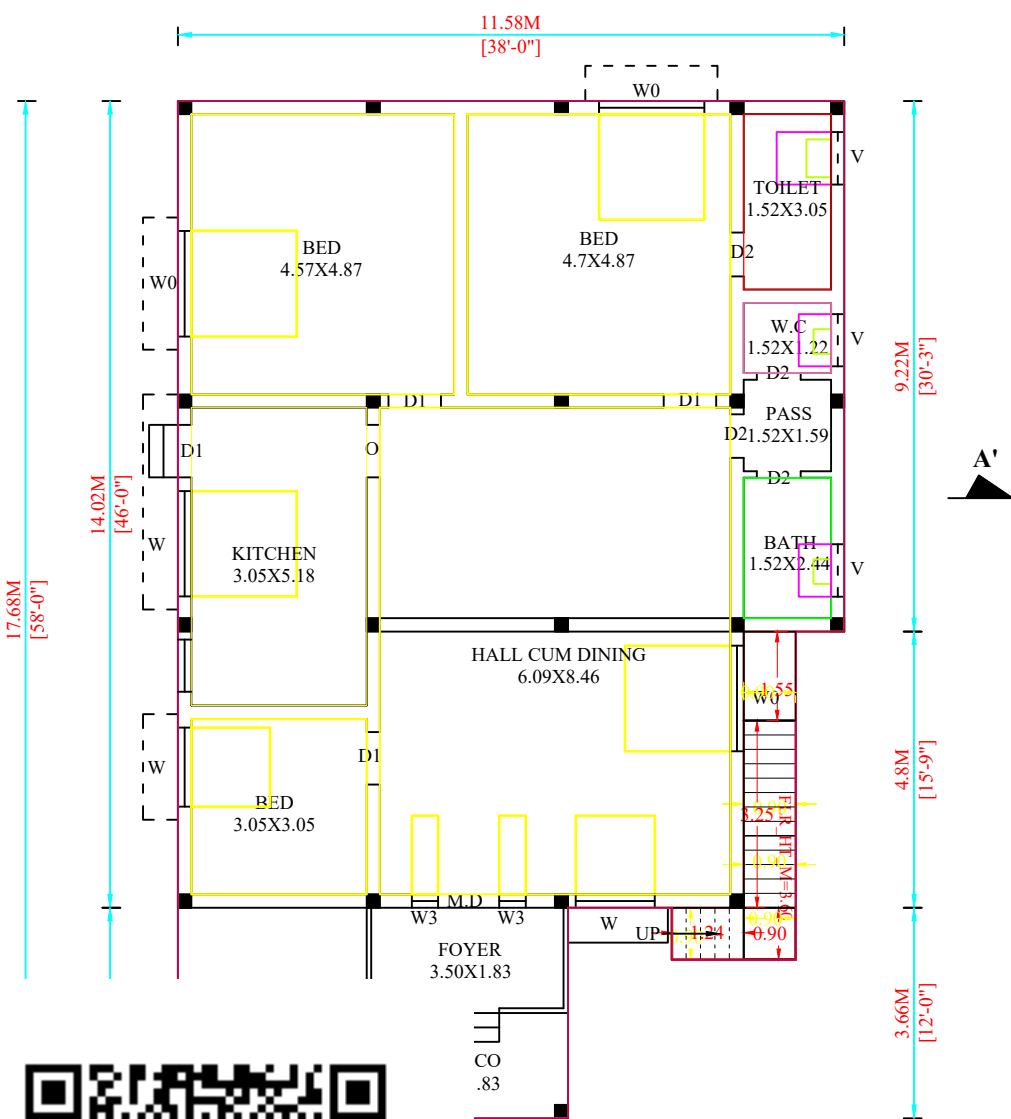
FLOOR PLAN
