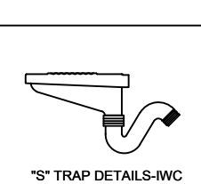
"S" TRAP DETAILS-IWC
