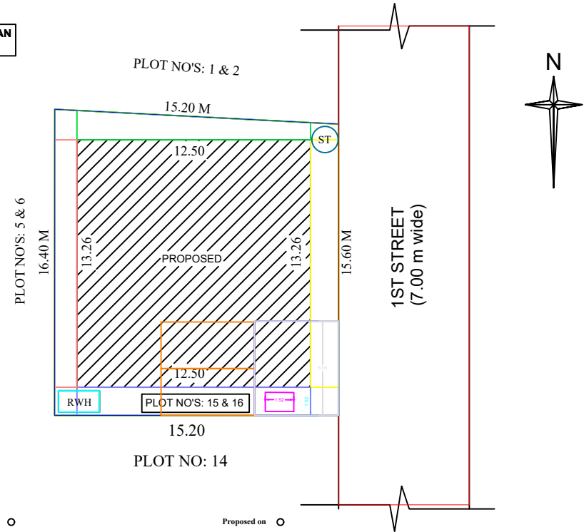
AREA DETAILS
