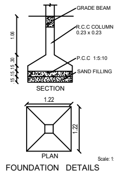
FOUNDATION DETAILS
