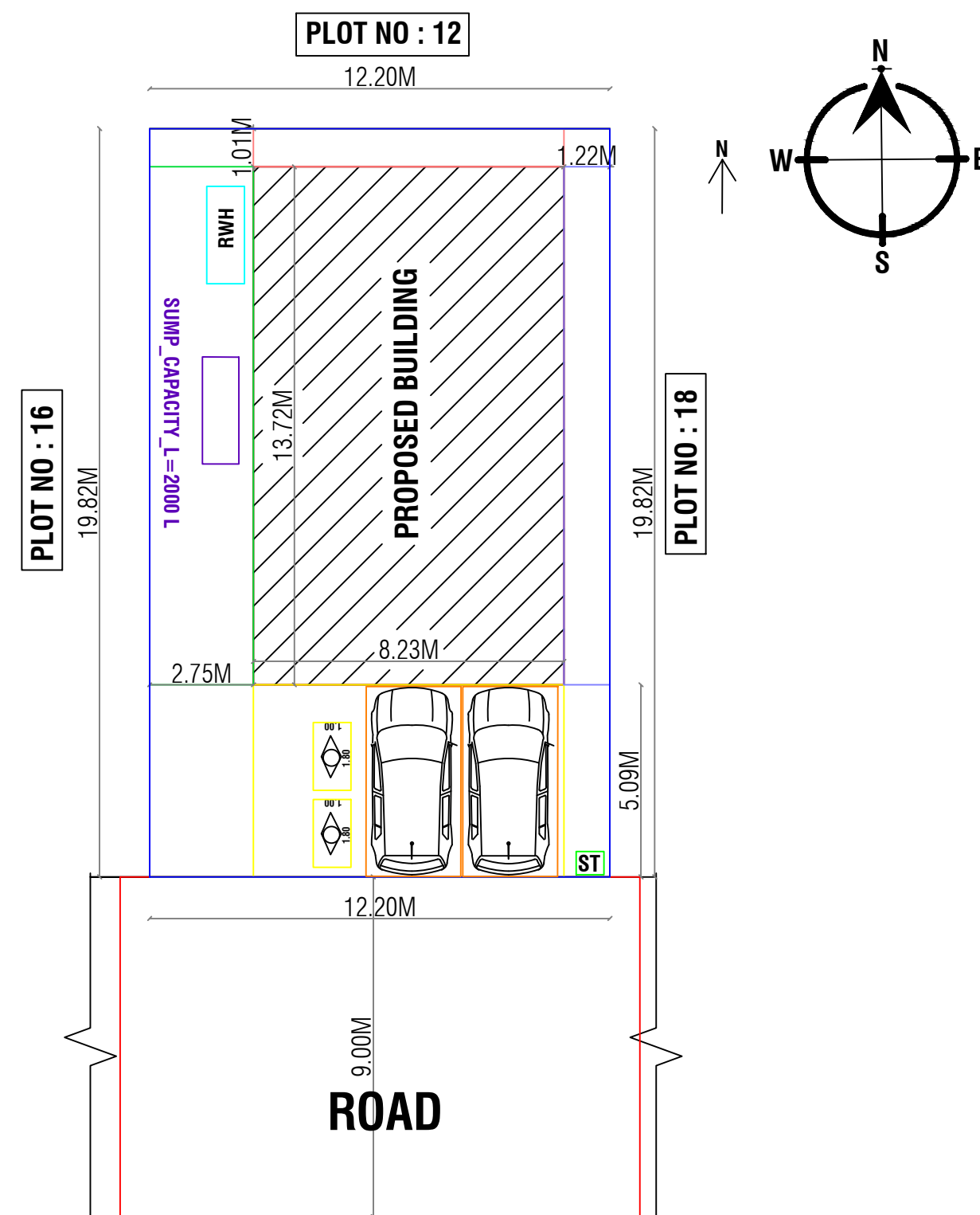
SITE PLAN
