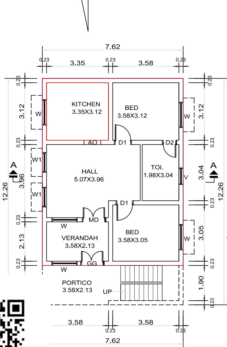
ROUND FLOOR PLAN
