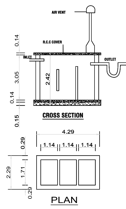
CROSS SECTION
