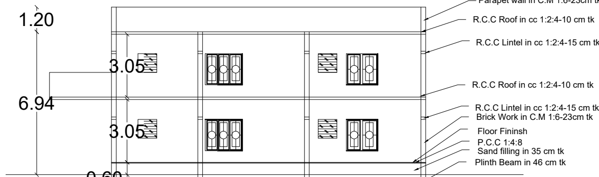
SECTION ON AR
