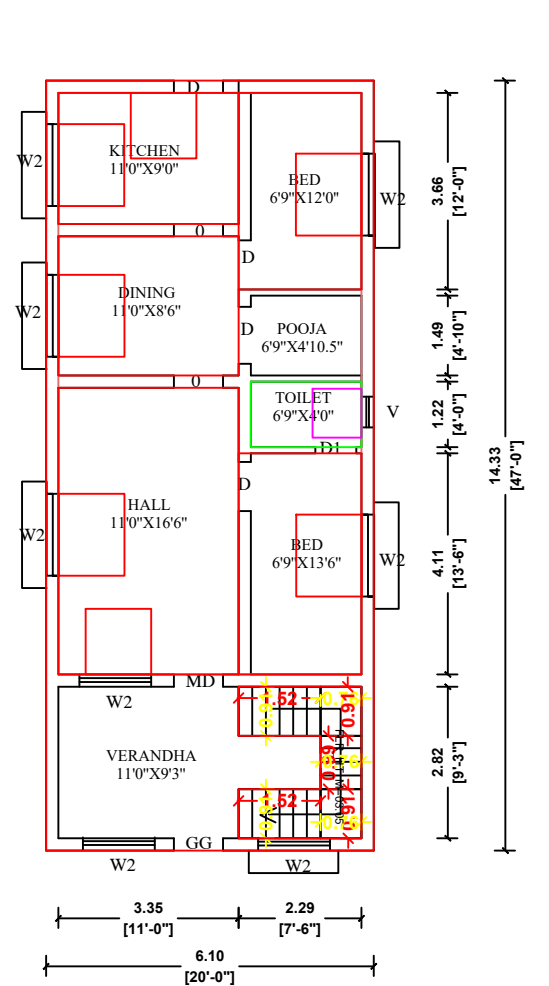
NORTH FACING PROPOSED GROUND FLOOR PLAN
