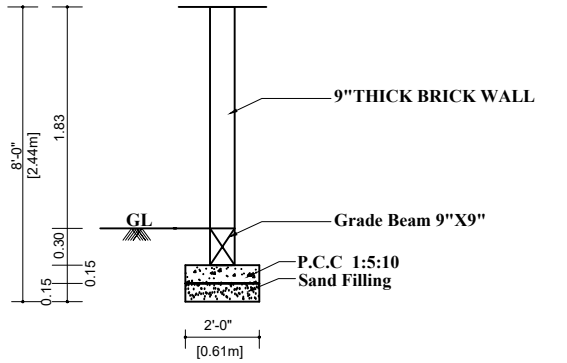
SECTION DETAIL (SCALE 1:50)
