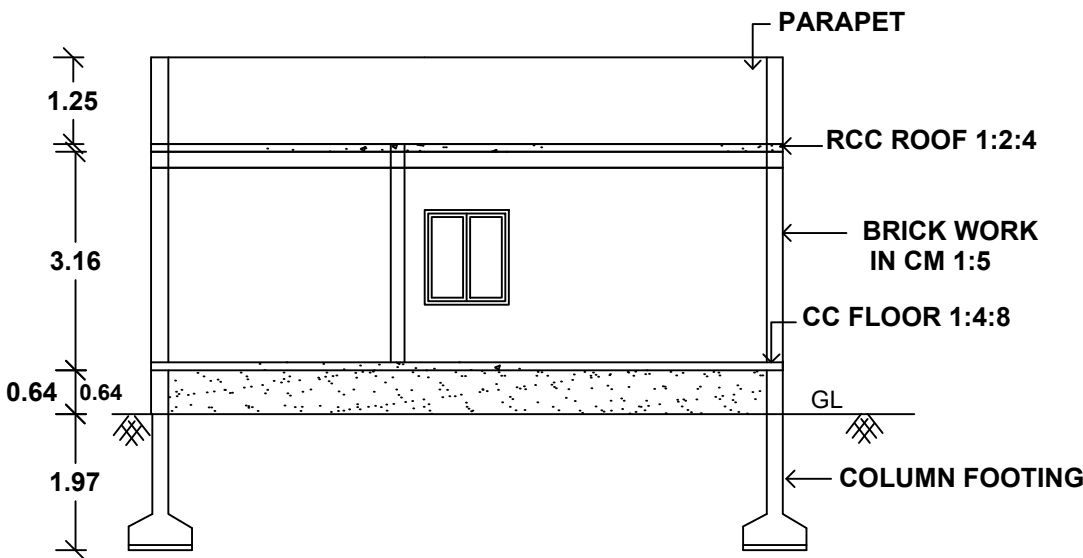
SECTION AB
