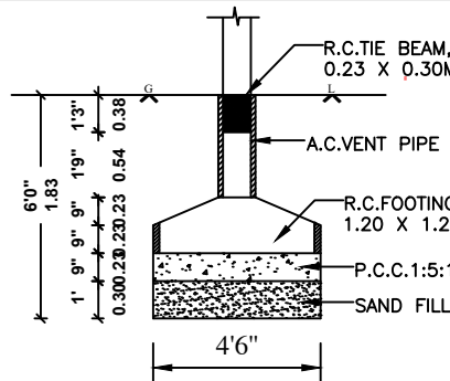
FOUNDATION DETAILS
