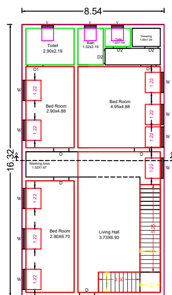
PRO.FIRST FLOOR PLAN
