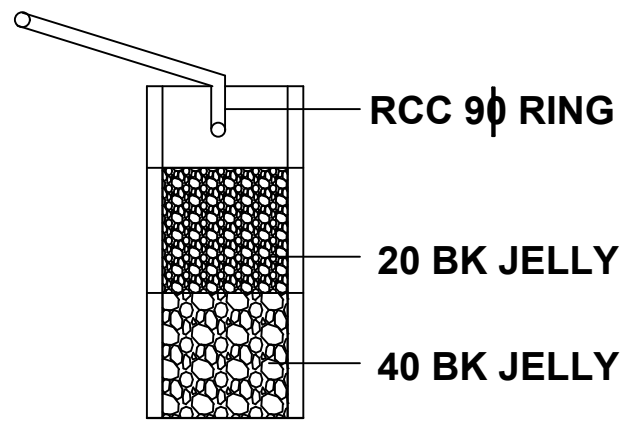
RAINWATER HARVEST PIT
