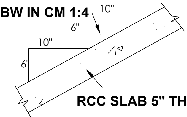
STAIR DETAIL
