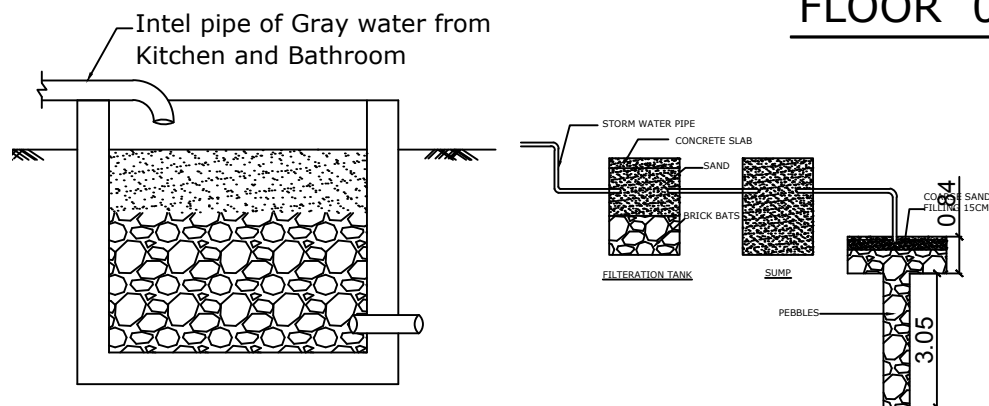
GREY WATER RECYCLING CHAMBER:-
