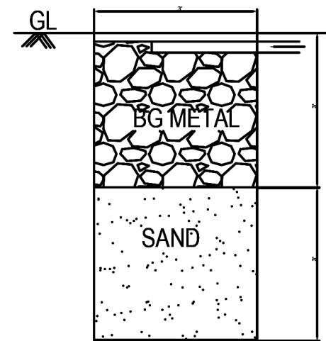
RAIN WATER HARVESTING PIT
