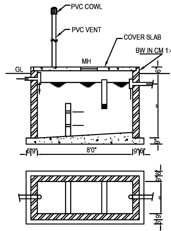
PLAN AND SECTION OF SEPTIC TANK
