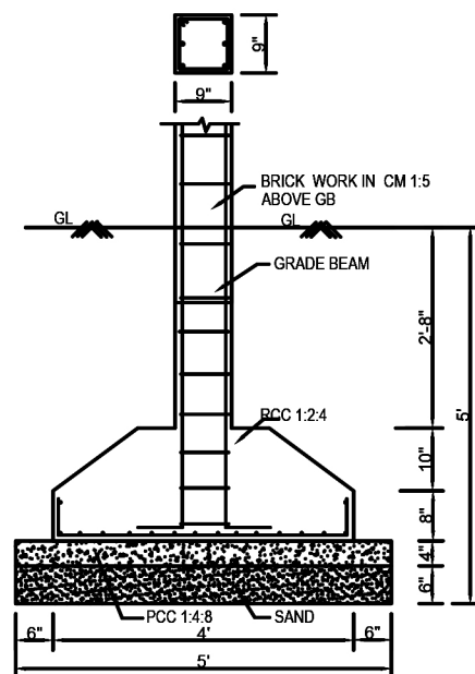
FOUNDATION DETAILS
