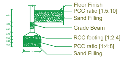
Foundation Details
