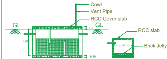
Section "AB"
