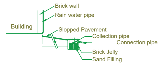
Details of Rain Water Harvesting pit
