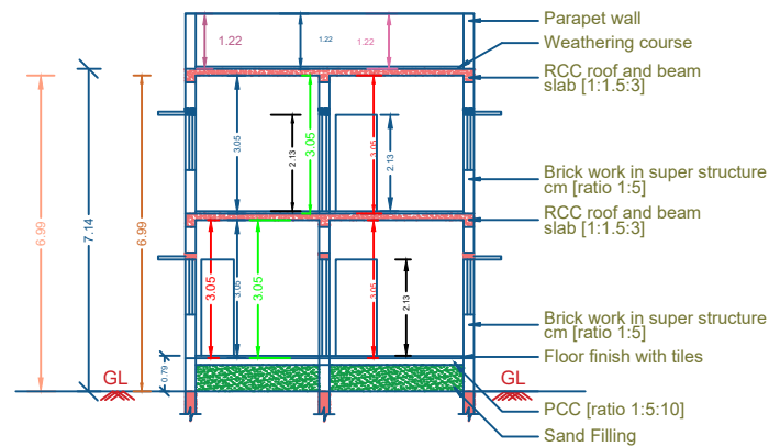
Section "AB"
