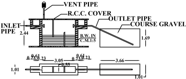
SEPTIC TANK & OF DISPERSION TRENCH DETAILS
