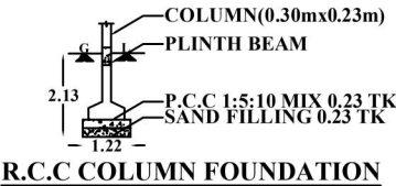
R.C.C COLUMN FOUNDATION
