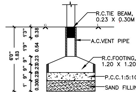
FOUNDATION DETAILS
