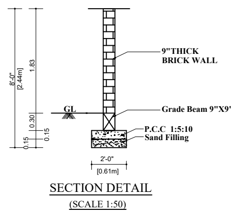
COMPOUND WALL DETAILS
