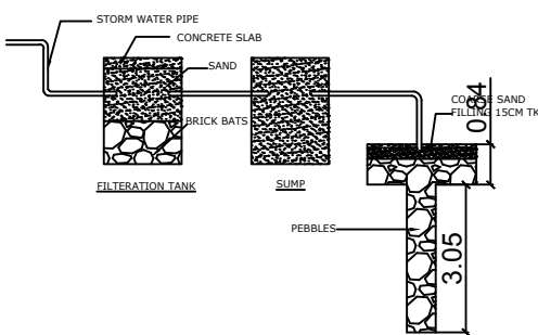
CONSTRUCTION DETAILS OF RECHARGE TRENCH
