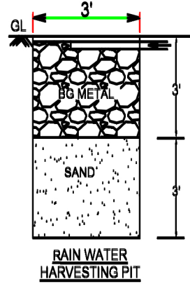
RAIN WATER HARVESTING PIT
