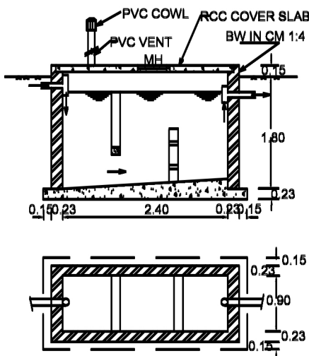
PLAN AND SECTION OF SEPTIC TANK
