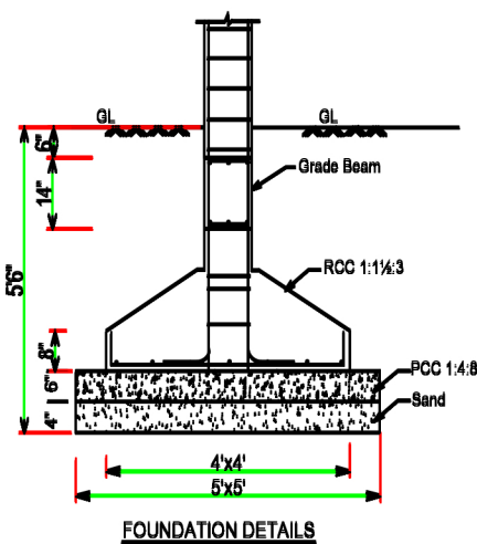
FOUNDATION DETAILS
