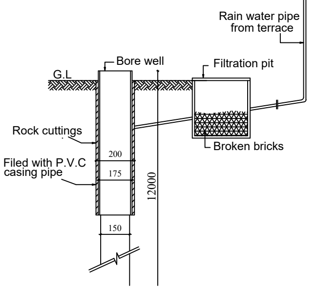
RAIN WATER HARVESTING DETAIL (not to scale)
