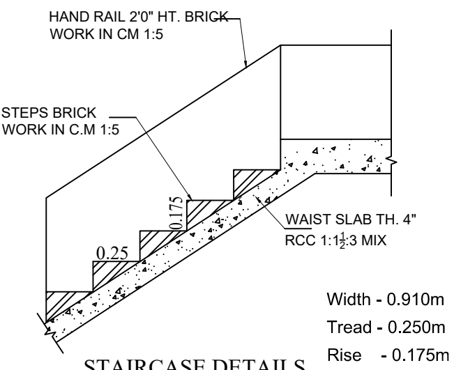
STAIRCASE DETAILS Scale (1:50)
