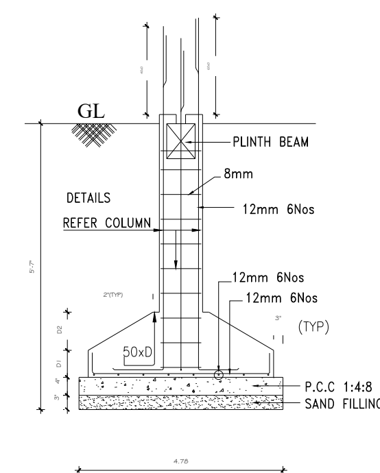
FOUNDATION DETAILS
