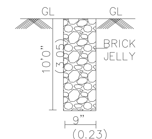
PERCULATION PIT
