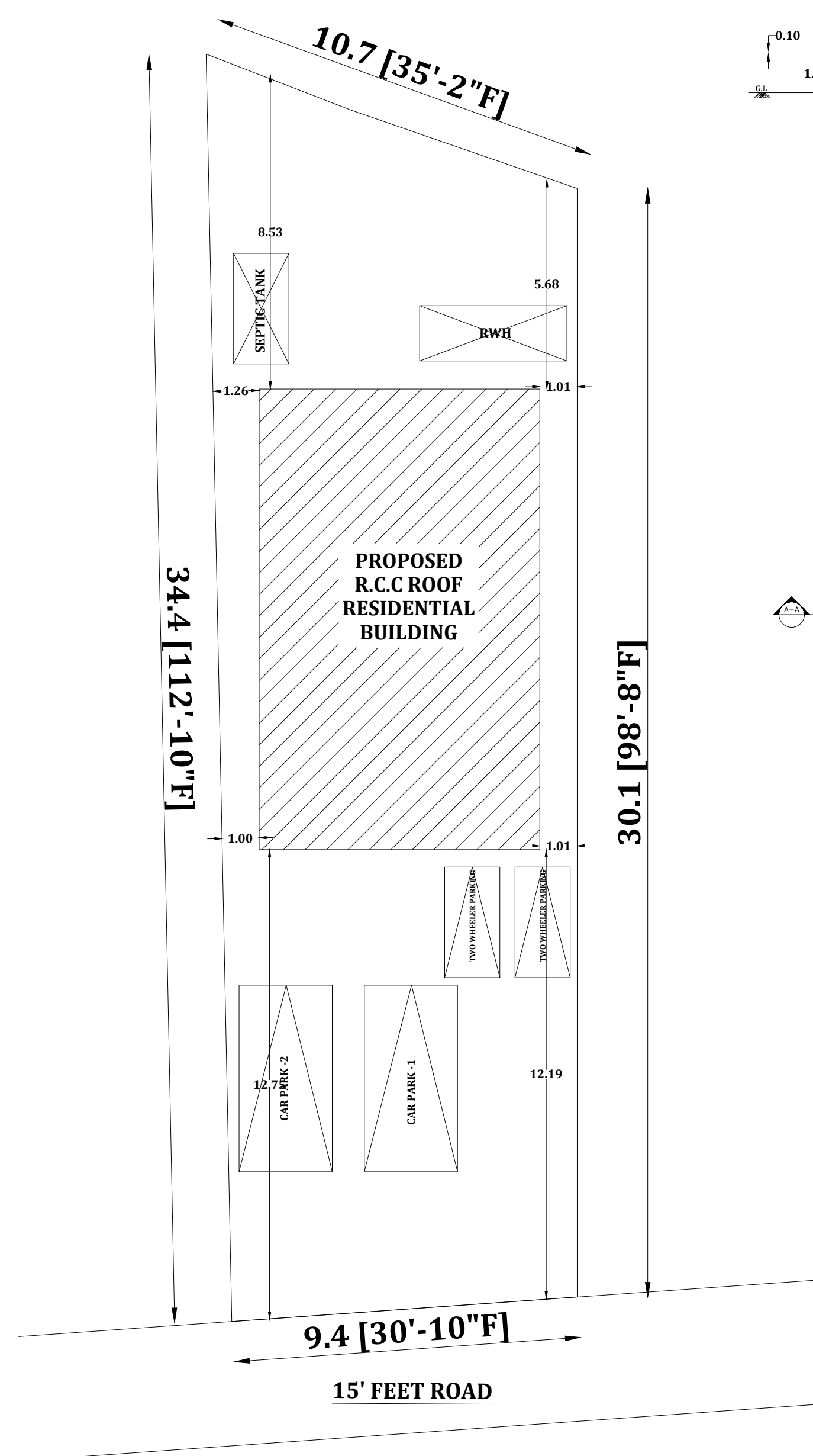
SITE PLAN
