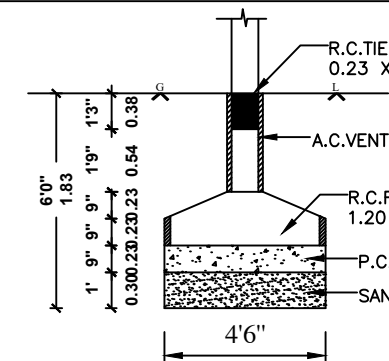
FOUNDATION DETAILS
