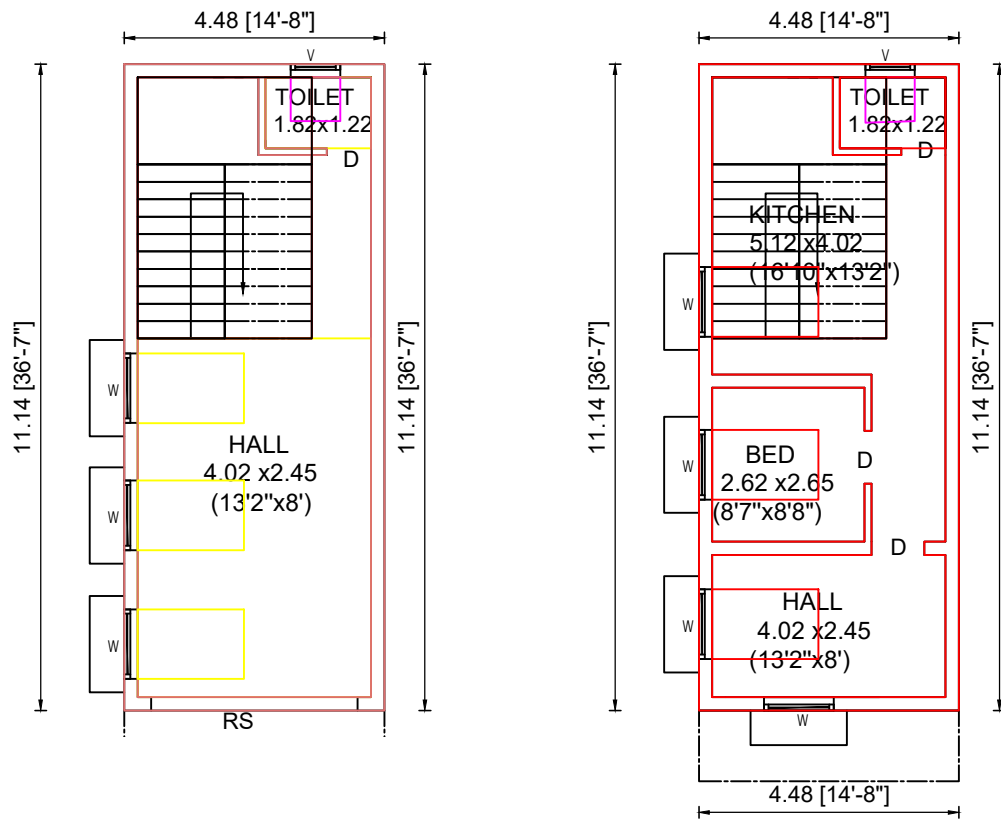
FIRST FLOOR PLAN- (NORTH FACE) HOUSE
