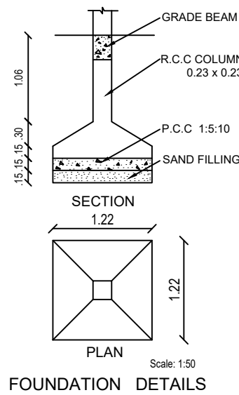
FOUNDATION DETAILS
