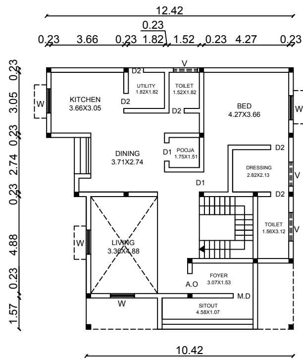
FLOOR 0
