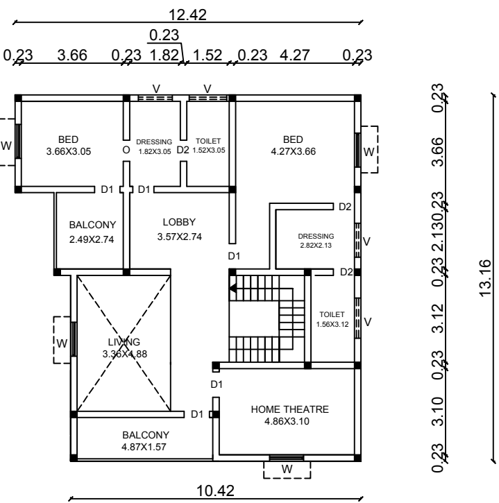
FLOOR 01
