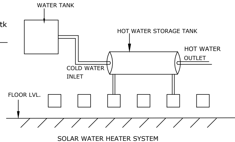
SOLAR WATER HEATER SYSTEM
