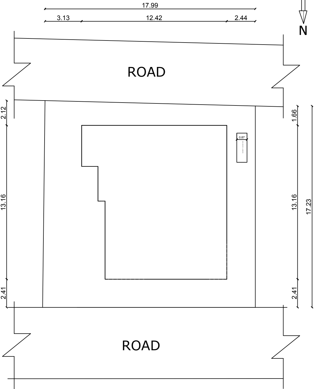
SITE PLAN
