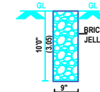
PERCULATION PIT
