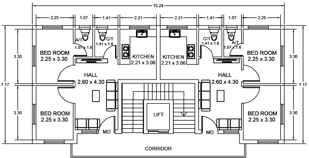
SECOND AND THIRD FLOOR PLAN
