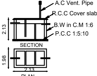
SEPTICTANK DETAILS
