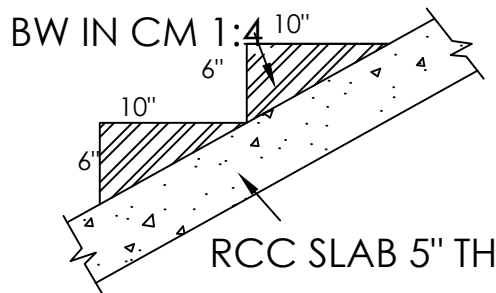
STAIR DETAIL
