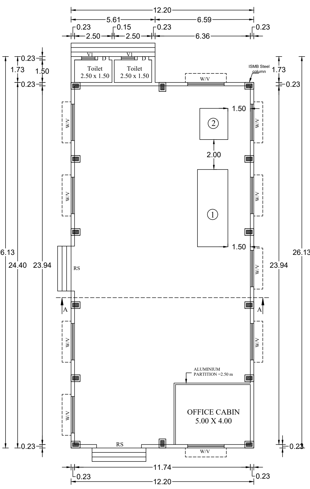
GROUND FLOOR PLAN PROPOSED (FACTORY BUILDING) SCALE - 1:100
