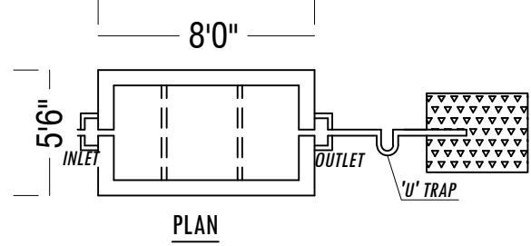
SEPTIC TANK AND DISPERSION TRENCH DETAILS
