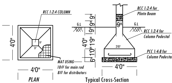
FOOTING DETAILS
