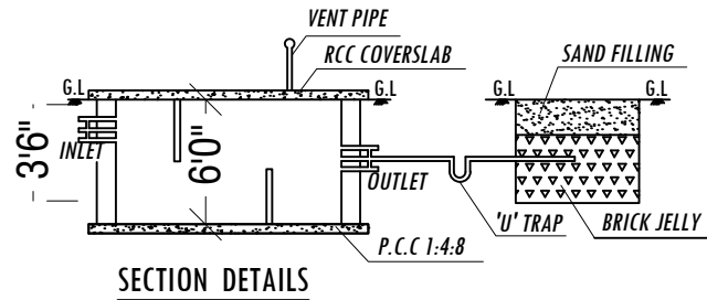
SECTION DETAILS
