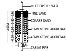
DETAILS OF RAIN WATER HARVESTING STRUCTURES
