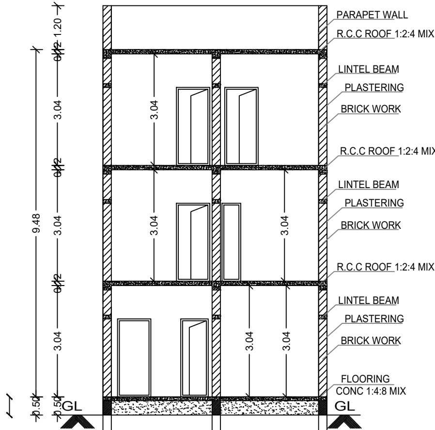
SECTION : "A-B"
