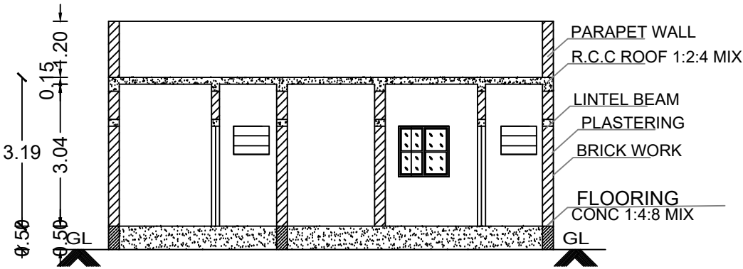
SECTION: A-B
