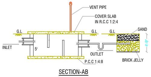
SEPTIC TANK & DISPERSION TRENCH DETAILS
