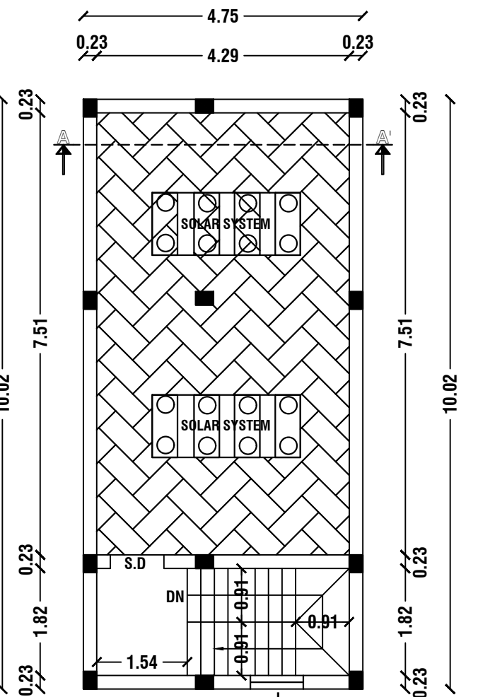
OPEN TERRACE FLOOR PLAN
