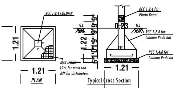
FOOTING DETAILS
