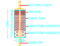
DETAILS OF RAIN WATER HARVESTING STRUCTURES
