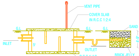
SECTION-AB
