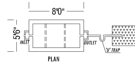
SEPTIC TANK AND DISPERSION TRENCH DETAILS
