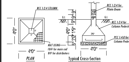
FOOTING DETAILS
