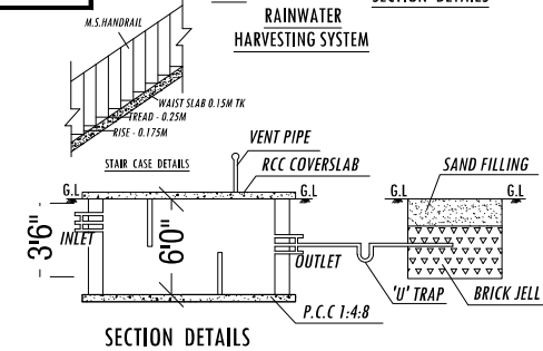
SECTION DETAILS
