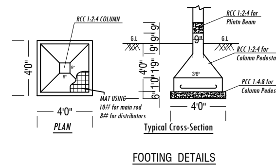
FOOTING DETAILS
