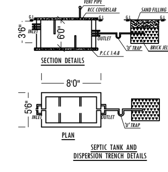
SECTION DETAILS
