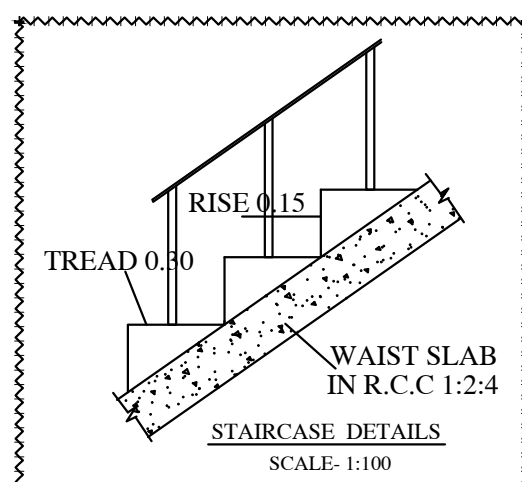
WAIST SLAB IN R.C.C 1:2:4 STAIRCASE DETAILS SCALE:1:100
