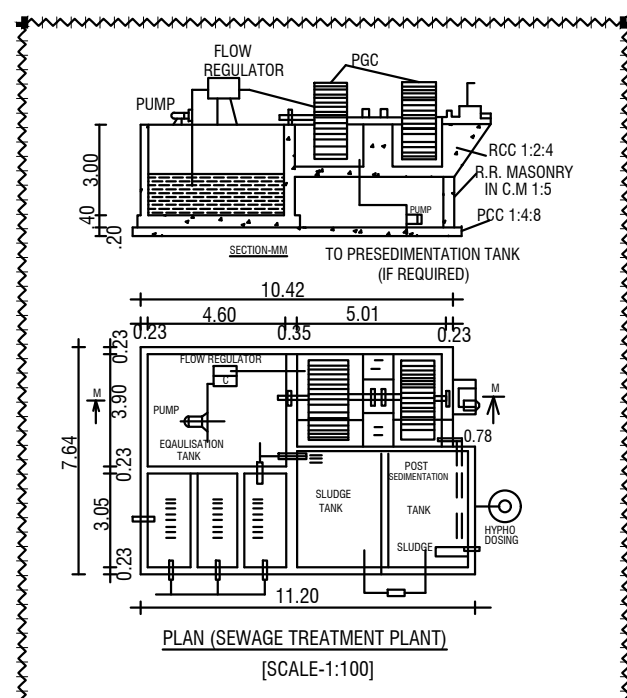
PLAN (SEWAGE TREATMENT PLANT) SCALE:1:100
