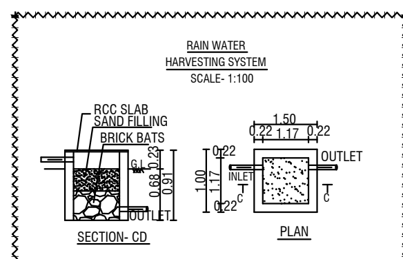
RAIN WATER HARVESTING SYSTEM SCALE:1:100
