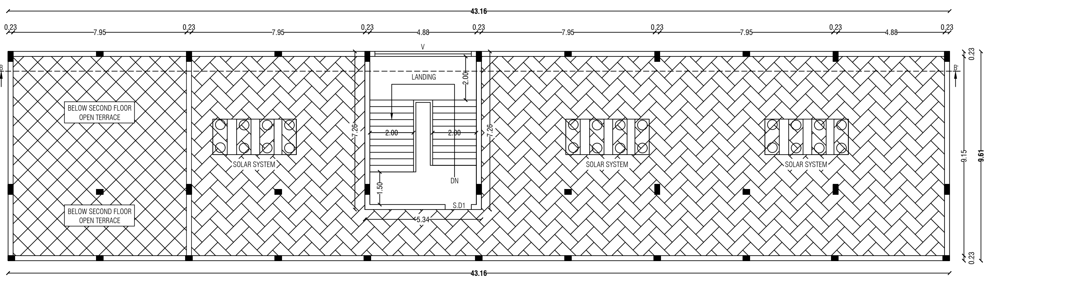
OPEN TERRACE FLOOR PLAN BLOCK - II PROPOSED
