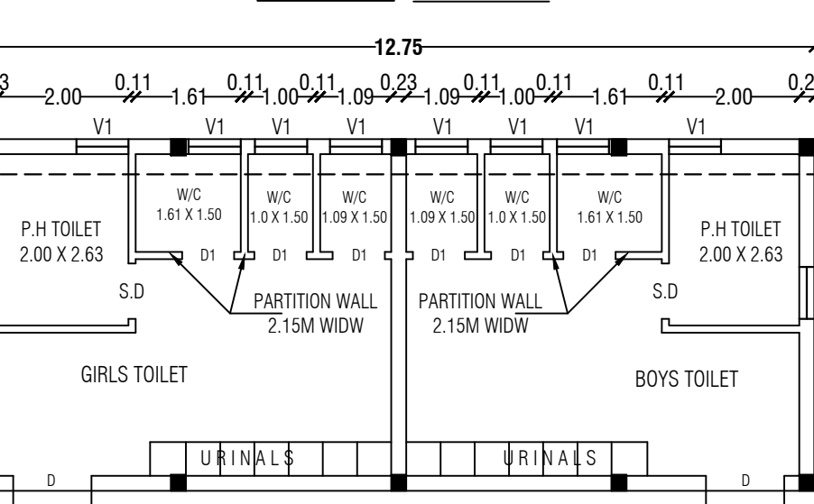
GROUND FLOOR PLAN PROPOSED TOILET BLOCK - III
