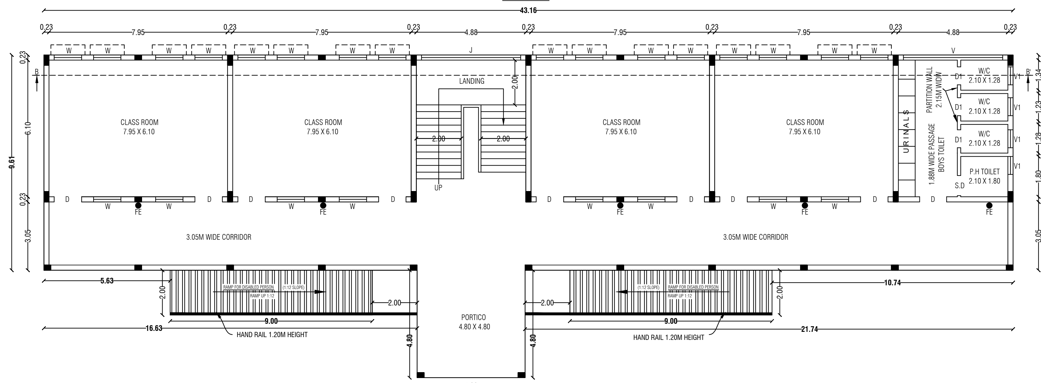
GROUND FLOOR PLAN BLOCK - II PROPOSED
