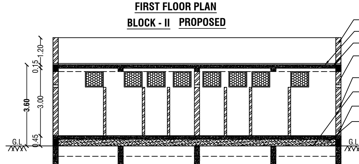
SECTION ON - CC' PROPOSED
