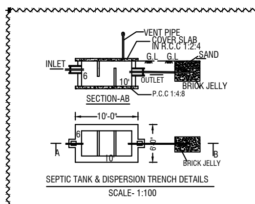
SEPTIC TANK & DISPERSION TRENCH DETAILS SCALE:1:100
