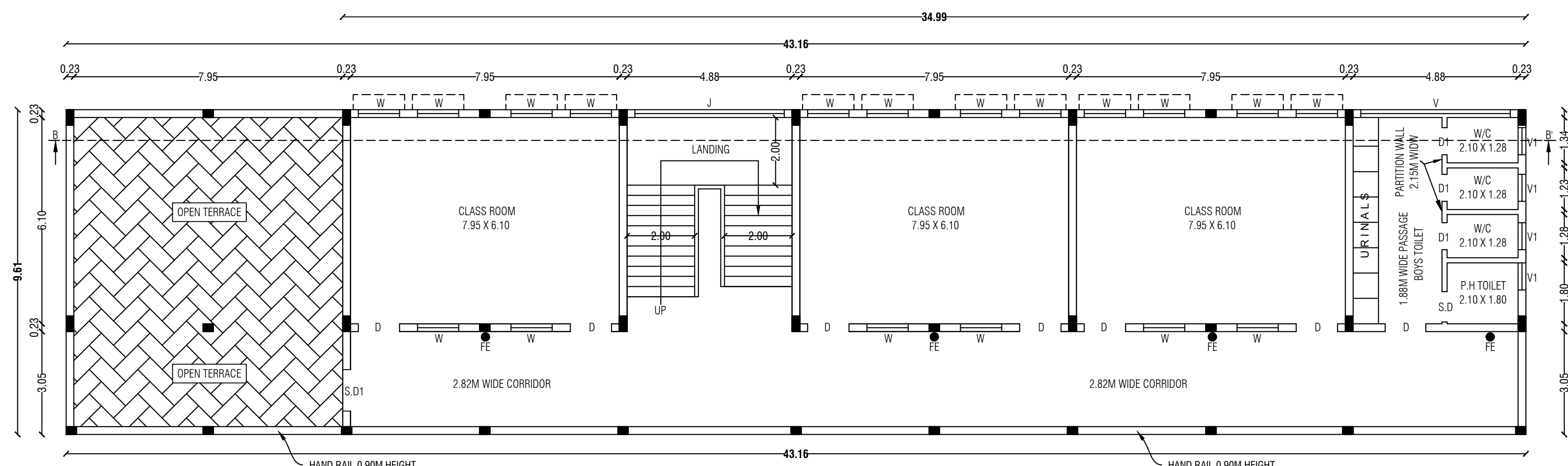
SECOND FLOOR PLAN BLOCK - II PROPOSED
