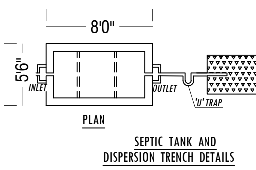
SECTION DETAILS
