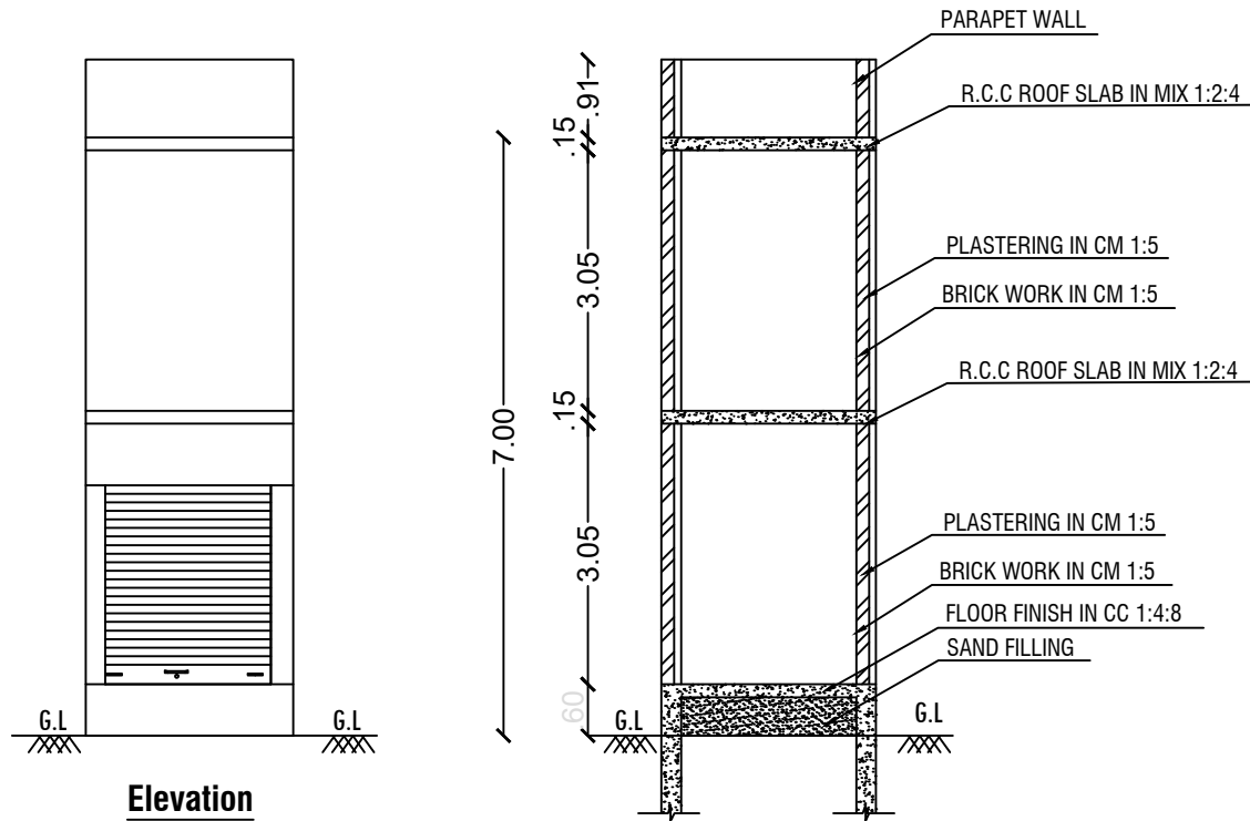
Section "US"
