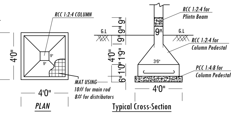
FOOTING DETAILS
