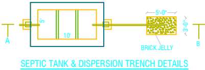
SEPTIC TANK & DISPERSION TRENCH DETAILS
