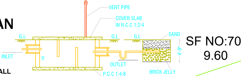
SECTION-AB
