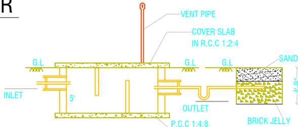
SECTION-AB
