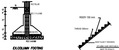
FOUNDATION DETAILS
