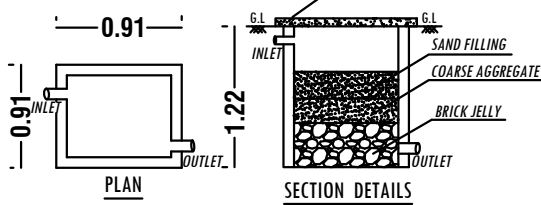
RAINWATER HARVESTING SYSTEM
