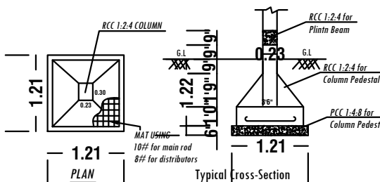
FOOTING DETAILS
